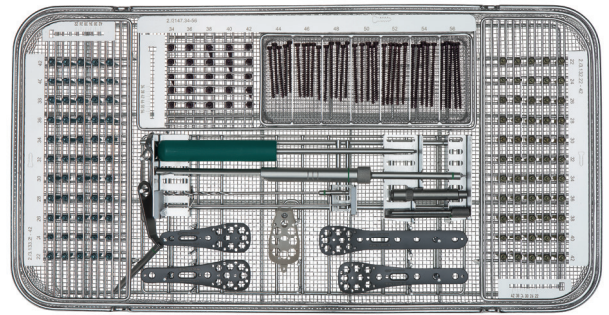
Set no. 19.3673.00 Internal hexagon
