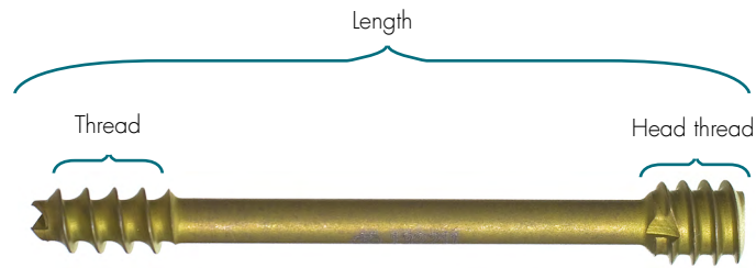
Fracture compressing screw Item no. 3.123.32
